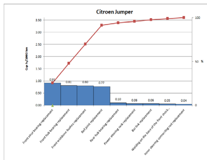
Fig. 2. Pareto chart for Citroen Jumper specific cost for failures elimination
