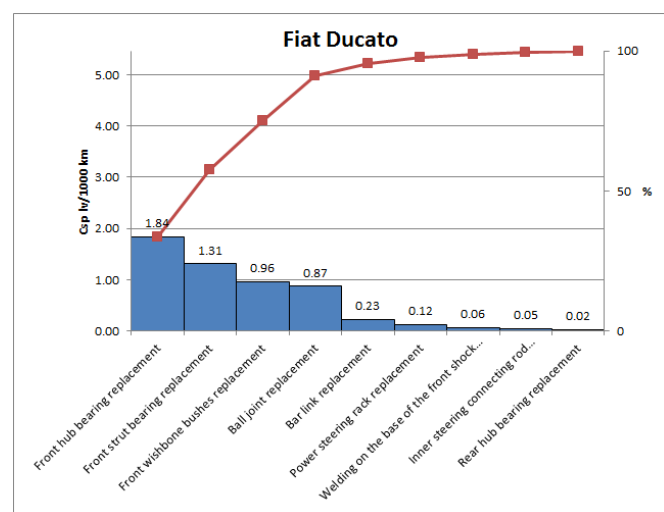
Fig. 3 Pareto chart for Fiat Ducato specific cost for failures elimination
