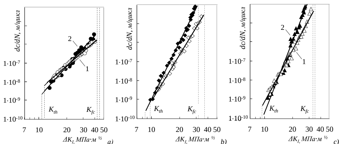
Fig. 3. Influence of operational medium on cycle crack resistance diagram for new (1) and used (2) metal (steel 10Г2БТЮ3) of "Druzhba" oil-trunk pipeline: a – laboratory air; b – distilled water; c – soil water
