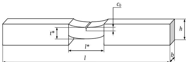
Fig. 1. The geometrical dimensions of the sample for developments fatigue failure investigation in pipeline steels
