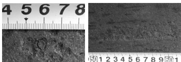
Fig. 2. Typical corrosion damages on "Druzhba" oil trunk pipeline internal surface
